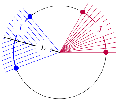
FIGURE 1. The configuration of lines in \mathbb{R}^2 for given arcs I, J .
