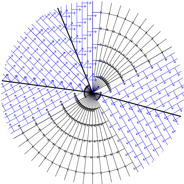
FIGURE 4. The calibration of C(I_1, \dots, I_k)
